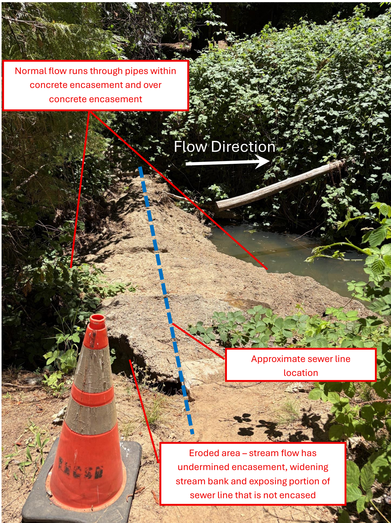
Existing Twain Harte Creek Sewer Crossing w/Concrete Encasement
